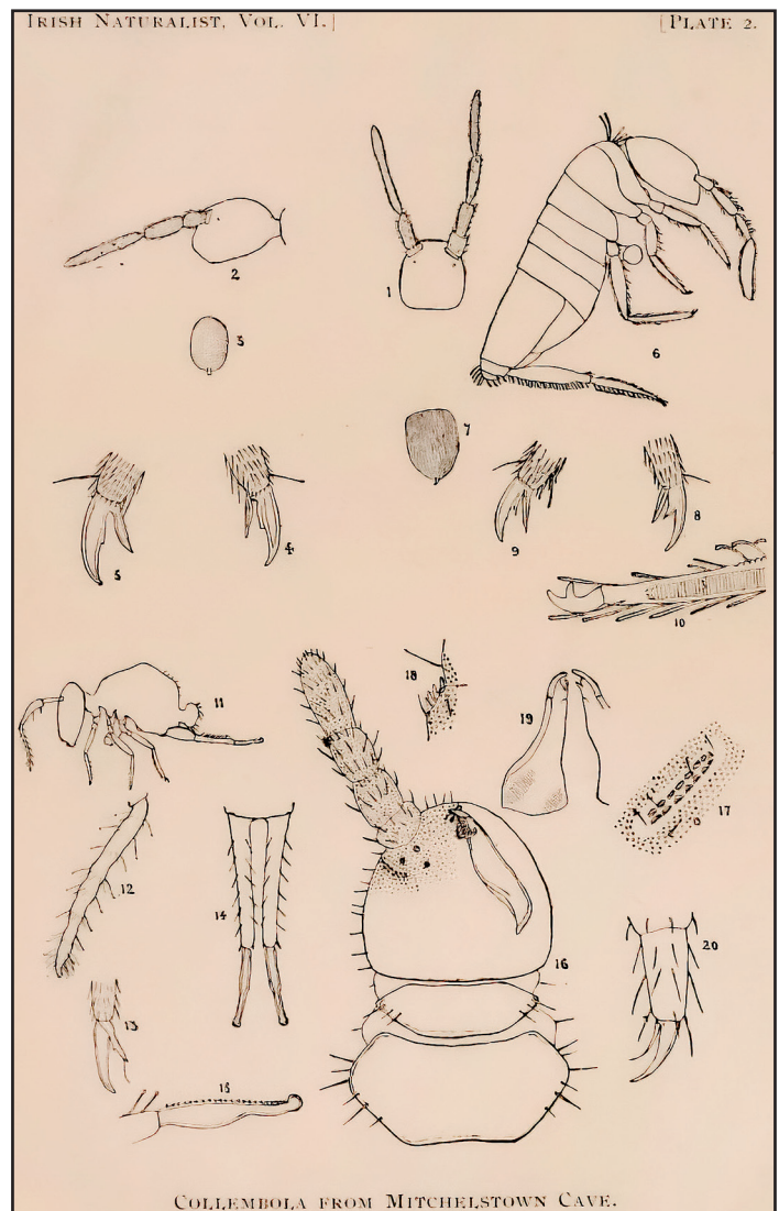
Figure 4: Collembola from Mitchelstown Cave. 1–5: Templetonia cavernicola , morphological details. 6: Cyphoderus Martelli , habitus; 7–10, morphological details. 11: Smynturus coecus , habitus; 12–15, morphological details. 16: Lipura Wrightii , habitus; 17–20, morphological details. [See Table 1 for updated taxonomy] [Reproduced from The Irish Naturalist , Vol.VI, No.9 (1897), Plate 2.]
