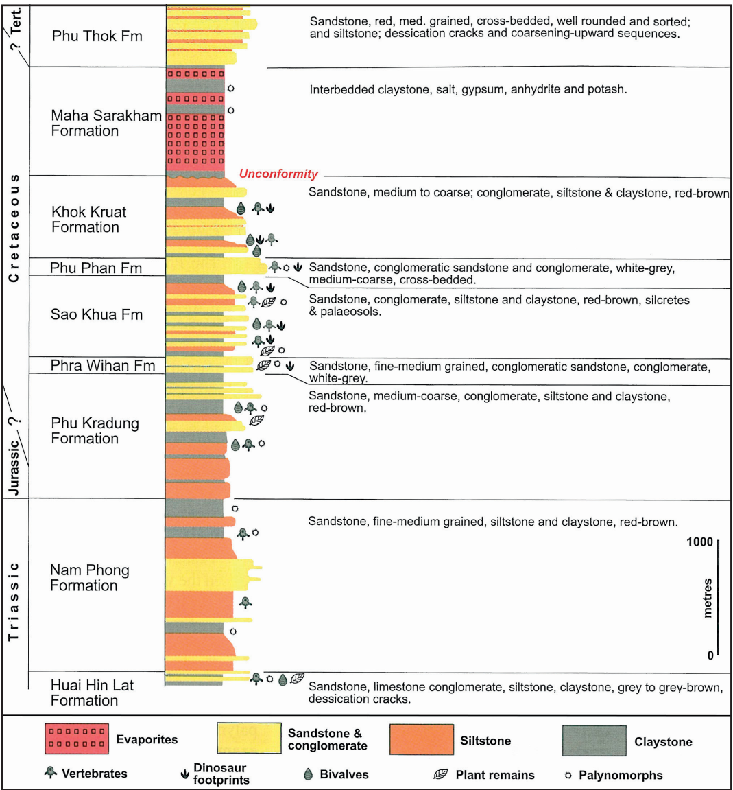
Figure 18: Mesozoic stratigraphical column of north-eastern Thailand. [After Meesook, 1999.]
