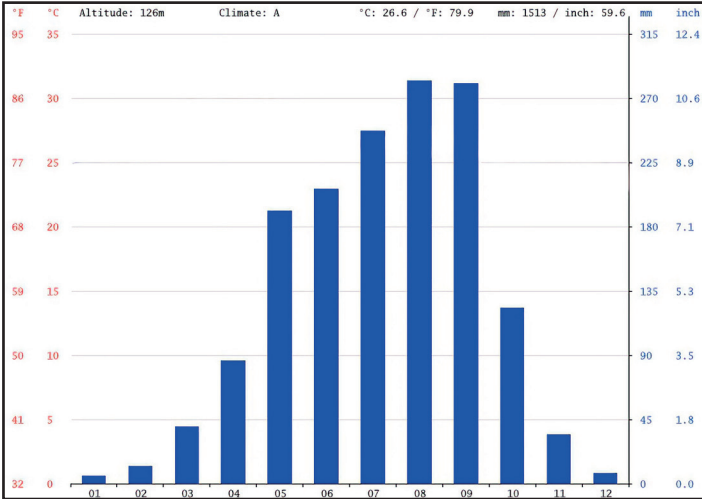
Figure 20: Average precipitation during 2003–2013 in Ubon Ratchathani Province (according to CLIMATE-DATA.ORG).
