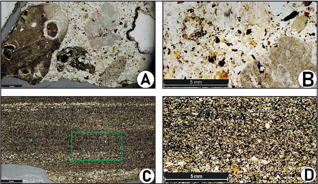
Figure 19 A–D: Photomicrographs of conglomerate and sandstone samples collected from the Phu Phan Formation on Mount Phu Pom. A; B: examples of two conglomeratic lithologies, both bound by a calcareous matrix/cement. C; D: a typical example of the quartzite sandstone within which the water pits occur. The rectangle drawn on image C indicates the approximate area that is shown at higher magnification on image D. Identified minerals include: quartz, feldspar, magnetite, haematite, tourmaline, zircon, calcite, and muscovite, cemented by syntaxial mineral overgrowths. Note: the scale bars on each of the four images represent 5mm. [Photos by TU Bergakademie, Institute of Geology, Freiberg.]
