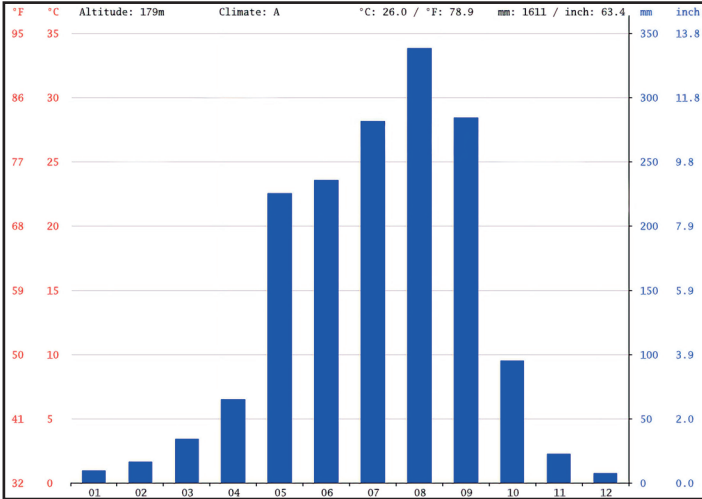
Figure 21: Average precipitation during 2003–2013 in Udon Thani Province (according to CLIMATE-DATA.ORG).
