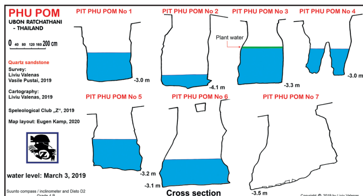
Figure 8: Sections through the 7 most important water pits at Phu Pom. [Cartography by Liviu Valenas.]
