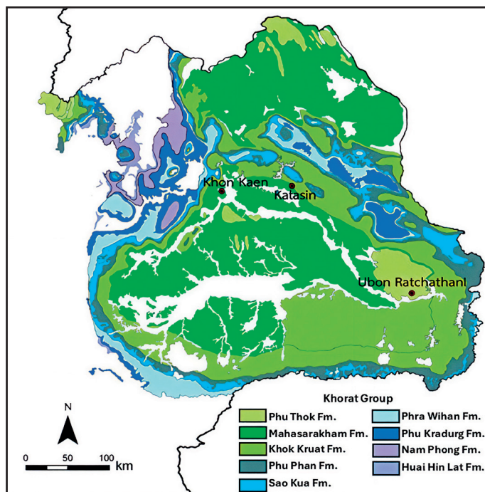
Figure 17: Geology of the Khorat Plateau. [from Wongklo et al. , 2019.]
