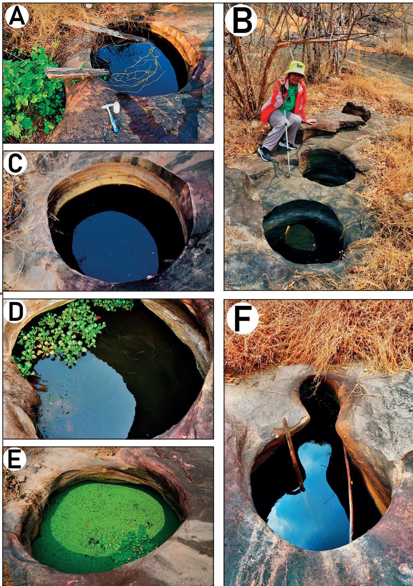
Figure 9A and 9C: Two typical water pits at Phu Pom with almost perfectly circular openings.
