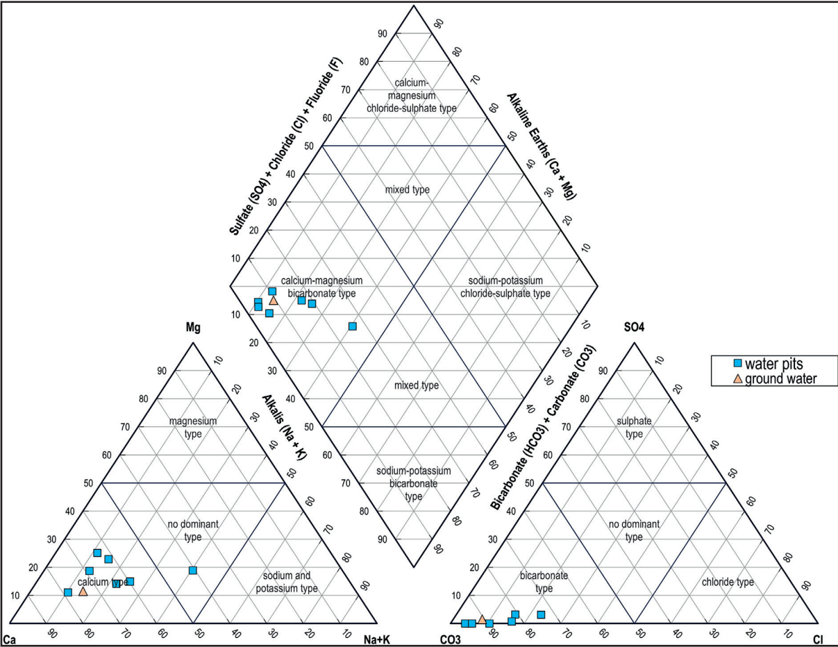
Figure 25: Piper diagram – prepared using the Excel template by Stosch (Version 1.1, 2022 – illustrating hydrochemical data of water samples from water pits (blue squares) and groundwater (orange triangles) in the study area. The cationic ternary plot (left) shows the relative proportions of calcium ( \text{Ca}^{2+} ), magnesium ( \text{Mg}^{2+} ), and the combination of sodium and potassium ( \text{Na}^+ + \text{K}^+ ), expressed as percentages of the total cations. The anionic ternary plot (right) similarly represents the relative proportions of chloride ( \text{Cl}^- ), sulphate ( \text{SO}_4^{2-} ), and the combined bicarbonate and carbonate ( \text{HCO}_3^- + \text{CO}_3^{2-} ) ions. Data points from both ternary plots are projected onto the central diamond field, which displays the overall hydrochemical facies of the water samples.
