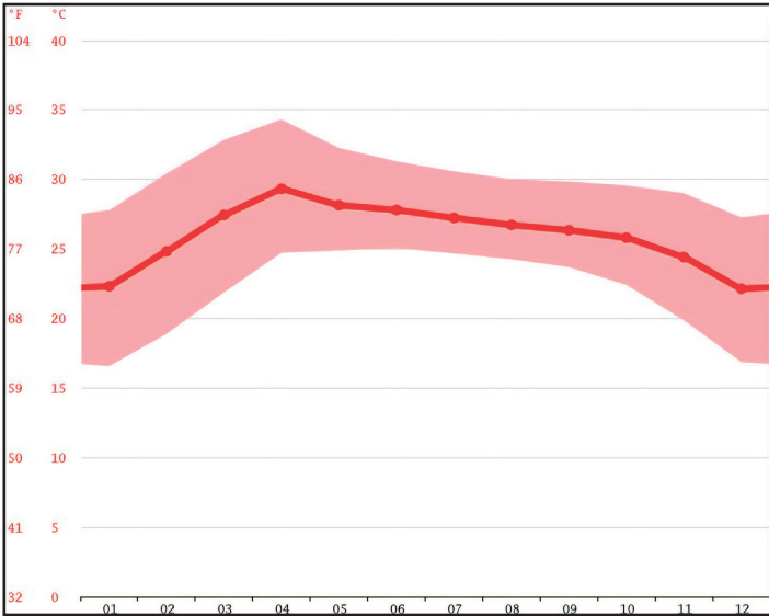
Figure 23: Average temperatures during 2003–2013 in Udon Thani Province (according to CLIMATE-DATA.ORG).
