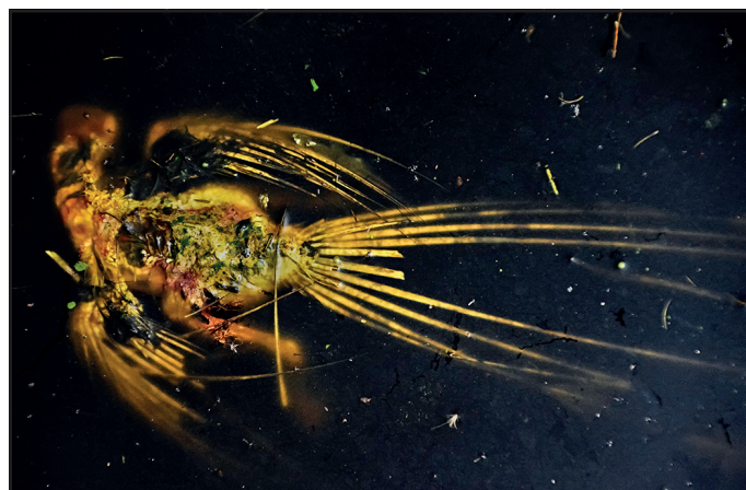
Figure 3: A relatively large bird remained trapped and died in a water pit at Phu Pom. This dead bird is directly responsible for a high concentration of ammonium in the water in this water pit. [Photo: Liviu Valenas.]
