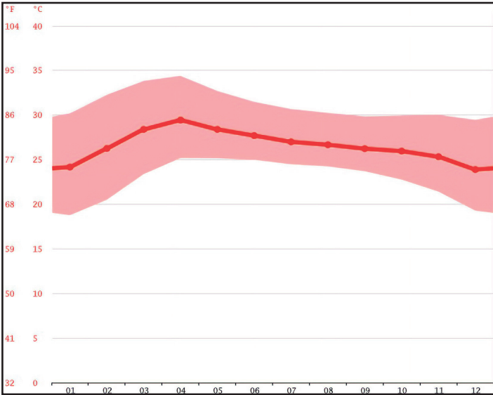
Figure 22: Average temperatures during 2003–2013 in Ubon Ratchathani Province (according to CLIMATE-DATA.ORG).
