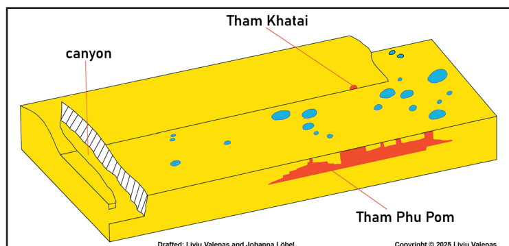
Figure 6: Block diagram of the Phu Pom plateau with water pits.
