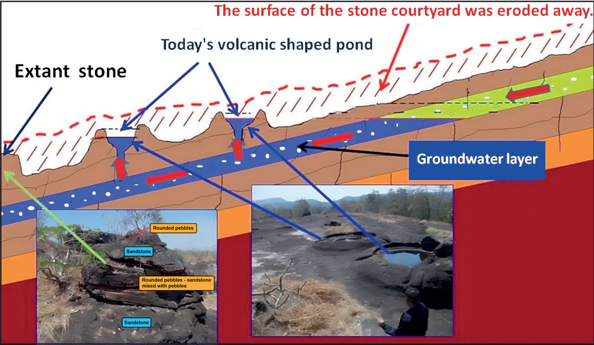
Figure 24: Model developed by the Department of Mineral Resources (DMR) Bangkok, to explain relationships at the Dong Luang water pits in Mukdahan Province. [Source: Facebook: Literal translations into English of the original Thai labelling are by Paradee Jinawan and Darin Gowland.] Note: The original figure includes the following text (translations as in the drawing) under the main panel: “The present remains can be seen that the surface of the stone courtyard has decayed. And was corroded and lost a lot until the shape was changed from the past.”
