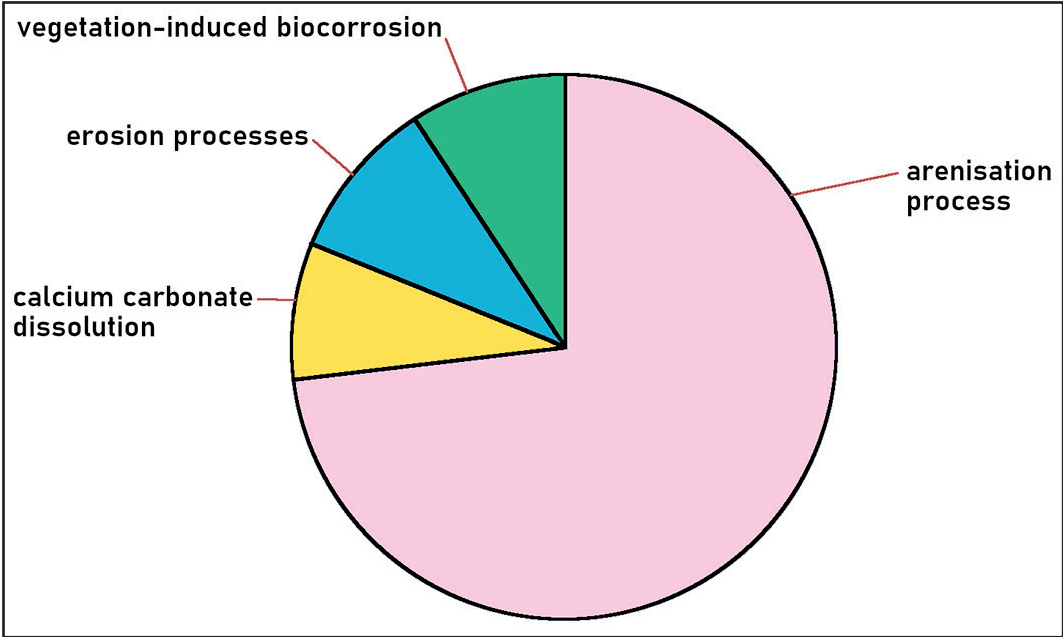
Figure 28: Model of the natural factors involved in the formation of the water pits on Mount Phu Pom.
