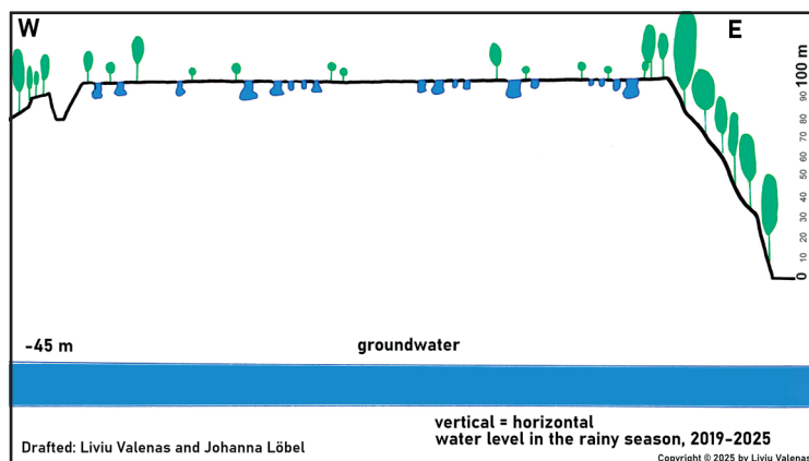
Figure 5: Profile of Mount Phu Pom. Note that the water pits at Phu Pom lie some 145m above the groundwater table. [Cartography: Liviu Valenas.]
