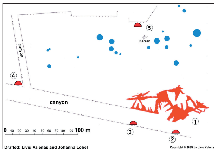
Figure 7: Map of the Phu Pom plateau with the 18 water pits. 1: Tham Phu Pom (284m total length), 2: Tham Phu Pom II (12m length), 3: Tham Phu Pom III (4m length), 4: Tham Phu Pom II (11m length), 5: Tham Khatai (3m length). The largest water pits of Phu Pom are aligned along west–east-oriented fault-related fractures, as are the main galleries of Tham Phu Pom. [Cartography: Liviu Valenas.]
