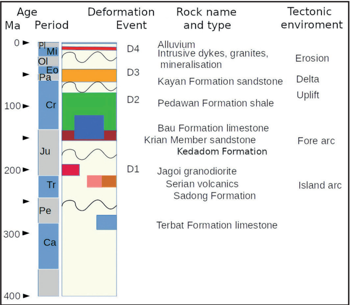
Figure 2: The geological sequence of the karst of southwestern Sarawak. [Compiled by Martin Laverty, after G E Wilford, and others.]
