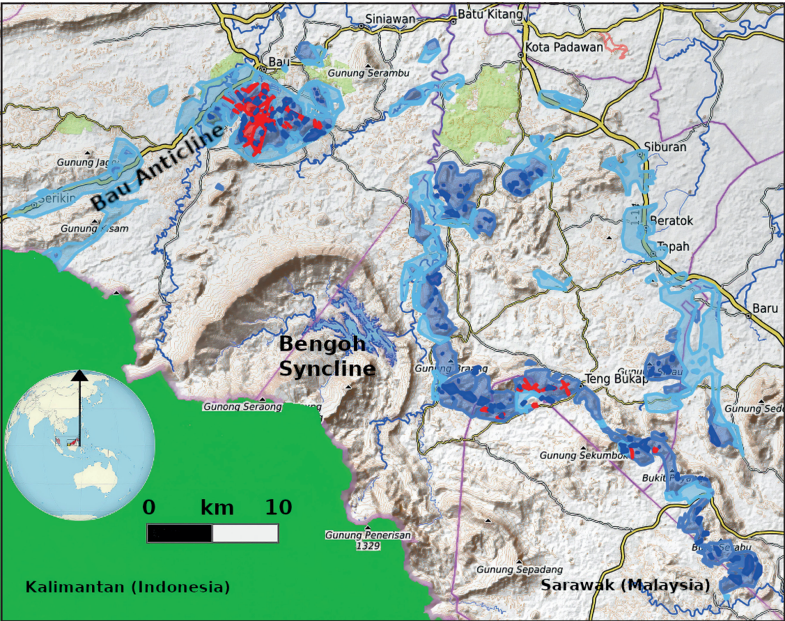
Figure 3: [OpenTopoMap base] with sketched details of: limestone hills (darker blue shades); depressions (darkest blue); limestone flats (paler blue shades), and main igneous intrusions (red) within the mapped limestone outcrops.
