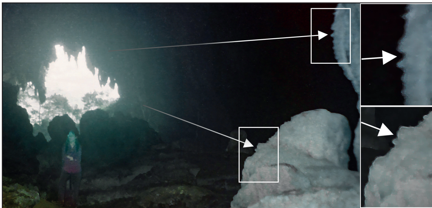
Figure 18: Delicate, acicular photokarren oriented towards the Fairy Cave entrance, which lies some 60m away.
