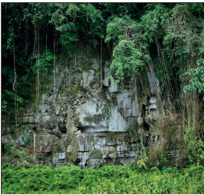
Figure 6: Cliff, with notches at various levels, near Kampung Skiat, Jambusan.
