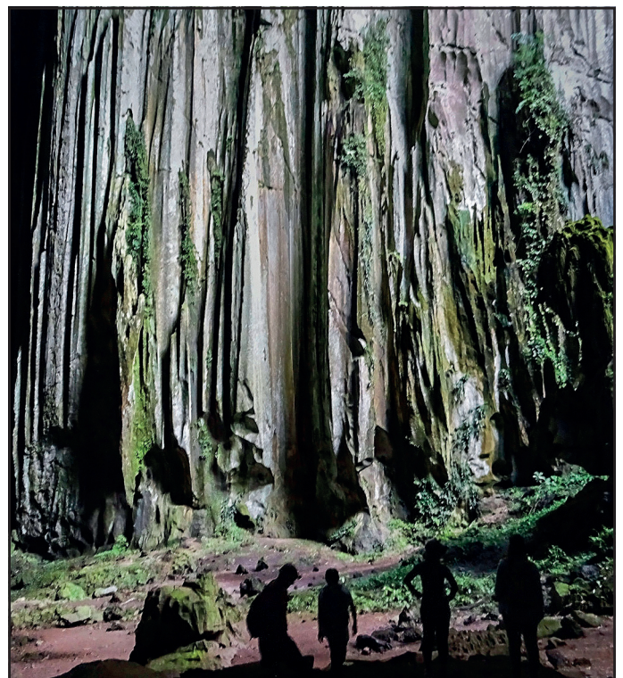
Figure 13: Apse-flutes soar upwards towards a ceiling opening in Gua Raya, Selabor.
