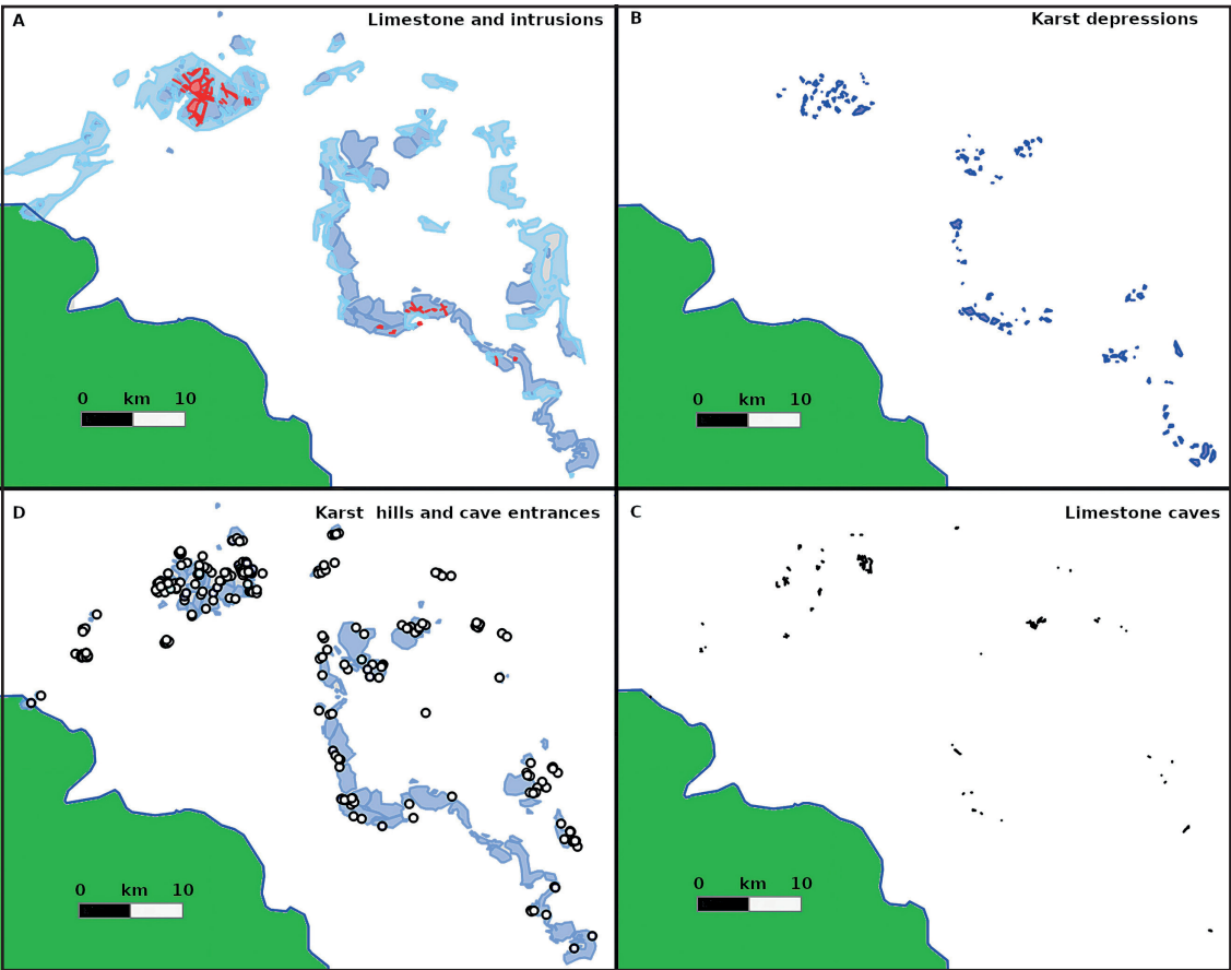
Figure 4: Sketch maps illustrating (clockwise from top left) the locations and known extent of: A: limestone hills (dark blue), limestone flats (pale blue), and igneous intrusions (red); B: karst depressions; C: cave passages; D: karst hills with currently recorded cave entrances (rimmed white circles).
